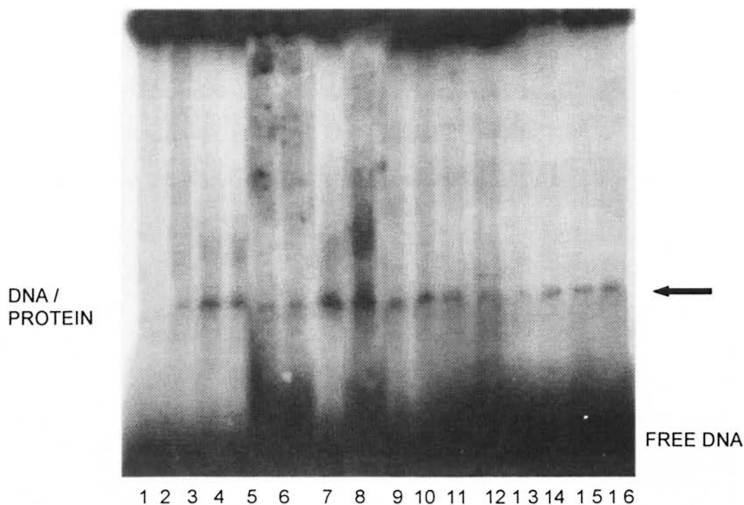
THE FIGURE. Gel Electrophoresis Mobility Shift Assays (EMSA) showing complexes formed between AP-1 consensus site \gamma - P^{32} labeled oligonucleotides (AP-1c) and nuclear extracts (NE) of lymphocytes from LL patients and healthy controls (HC) subjects: Lane 1: Control without NE; lane 2: HeLa cell control NE; lanes 3–6: AP-1c + NE from cells of HC; lane 7–16: AP-1c + NE from cells of LL patients. Lanes 3, 5, 7, 9, 11, 13, 14 complexes of AP-1c + NE from cultures with medium. Lanes 4, 6, 8, 10, 12, 15, 16 complexes of AP-1c + NE from cultures stimulated with PHA.
